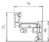
Flügel 70mm nitr. ★ 103.296 Stahl 113.291
